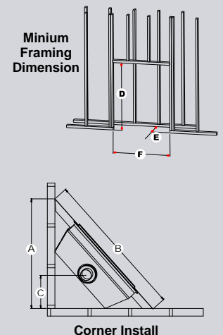
Framing Dimensions
